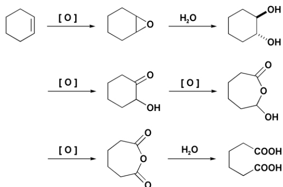
Fig. 15 Direct oxidation of cyclohexene to adipic acid.
