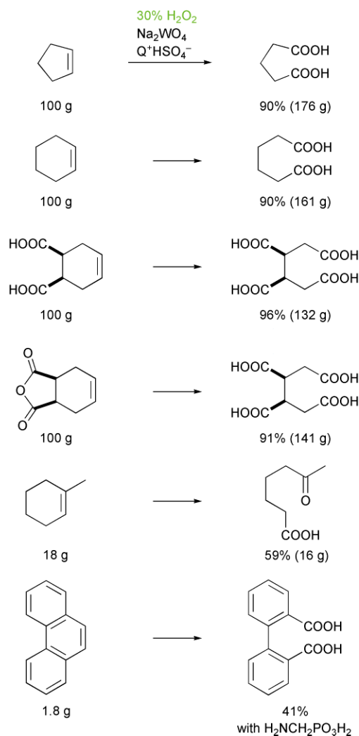
Fig. 16 Oxidative cleavage of cycloolefins.
