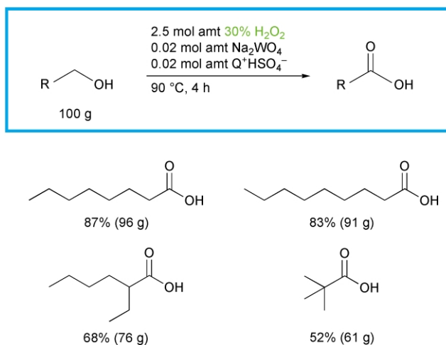
Fig. 3 Oxidation of primary alcohols to carboxylic acids.
