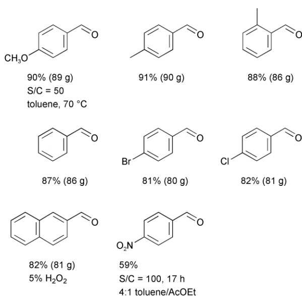
Fig. 6 Oxidation of arylcarbinols to aldehydes.
