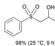
Fig. 17 Oxidation of sulfides to sulfones.
